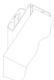
PD-2 Aluminiumskarm Fast karm for veggykkelser fortrinnsvis over 300 mm
